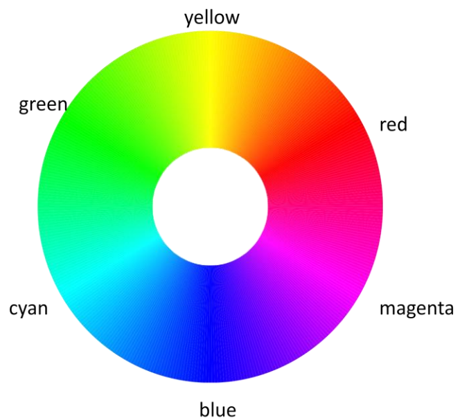
Colour Wheel
