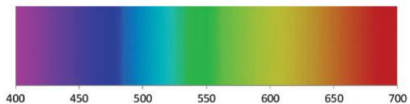
The Visible Spectrum
