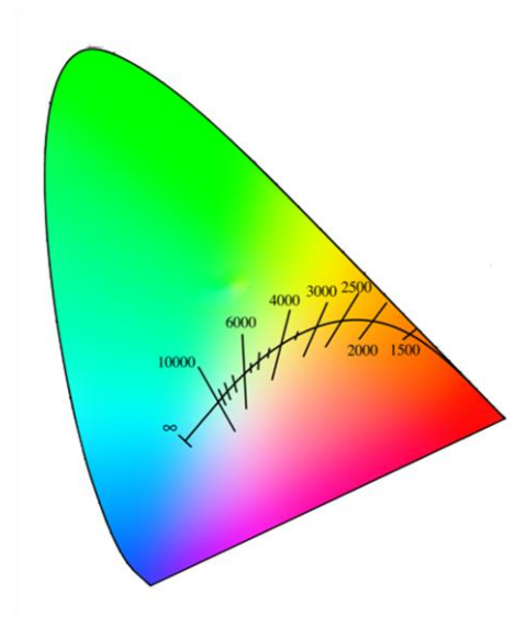
CIE diagram showing the Colour Temperature scale
