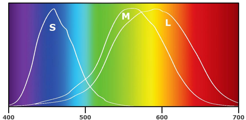
The Response of the Human Eye
