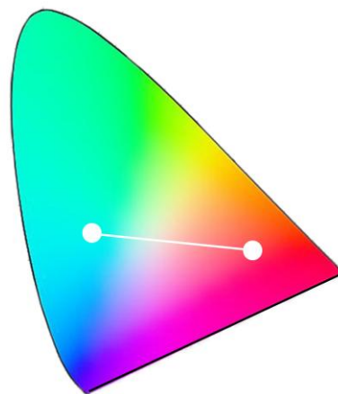
The colours you get by mixing two colours lie on a straight line between those colours.
