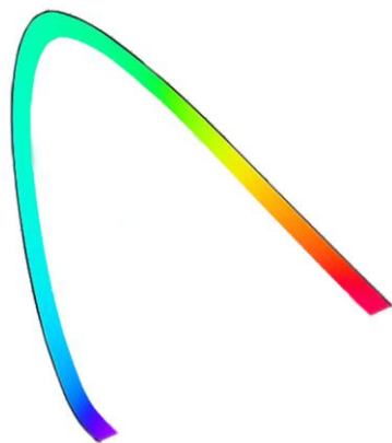
Horseshoe made by bending the Visible Spectrum
