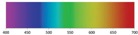
The Visible Spectrum
