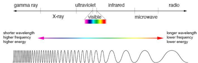
The Electromagnetic Spectrum
